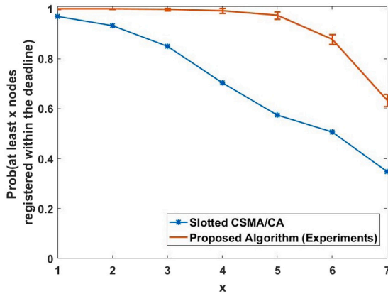
Fig. 3. Comparison between the proposed Device Registration Algorithm and slotted CSMA/CA with 7 nodes in the network and a deadline of 49 ms.
