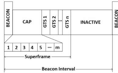
(b) Modified superframe structure which shows the division of CAP into microslots.
