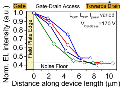
Figure 5. Normalized EL intensity of different devices with critical voltage < 170 V depicting an EL intensity peak near field plate edge.
