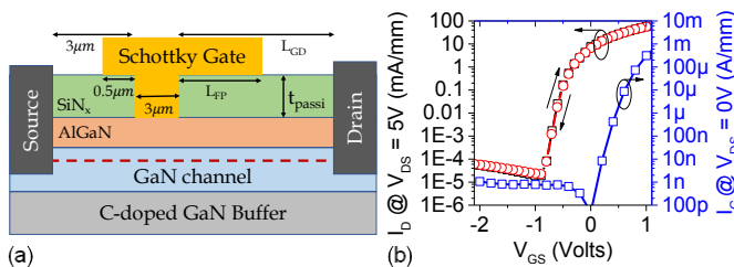
Figure 1. (a) Fabricated Schottky gated AlGaN/GaN HEMT on commercial 600-V stack. (b) Transfer and gate leakage characteristics depicting negligible hysteresis & low leakage current demonstrating excellent surface and interface quality.
