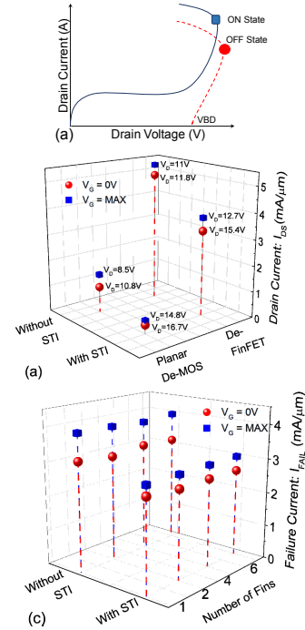
Figure 9: Comparison of Safe operating area (SOA) of DeFinFETs and Planar DeMOS (a) SOA of drain extended devices are extracted using the failure current: I_{t2} . at ON state V_{GS} = V_{Gmax} and OFF state V_{GS} = 0V . (b) Extraction method used to define SOA. SOA covered by the DeFinFETs is 5x times higher than its planar DeMOS counterpart. (c) SOA is independent of the multifinger arrangement in DeFinFETs, which makes them more suitable for HV integration over planar DeMOS devices
