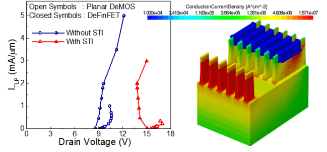
Figure 8: (a) TLP IV characteristics of Planar DeMOS (w/ and w/o STI). (b) Uniform current conduction during ESD stress in multifin configuration of DeFinFET.
