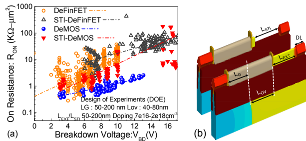
Figure 3: Performance Metric: (a) On Resistance ( R_{ON} ) vs Breakdown Voltage ( V_{BD} ) of DeFinFET and STI-DeFinFET devices. (b) 3D view of DeFinFET depicting channel length ( L_G ), Overlap Length ( L_{OV} ), Drift Length ( L_{EXT}/L_{STI} ) and drain contact length (DL).
