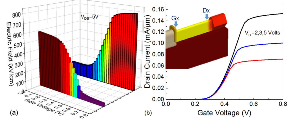
Figure. 4 (a) Quasi Saturation (QS) depicted through a shift in the peak electric field as a function of V_{GS} . Here Gx and Dx are referred to the position at Gate and Drain edge respectively as shown in the inset of (b), (b) transfer characteristics of DeFinFET depicting severe Quasi-Saturation at different Drain biases, is attributed to inevitable narrow fin architecture.
