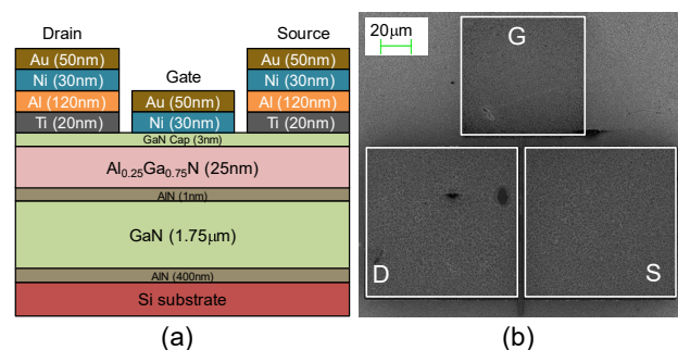
Figure 1. (a) Schematic view of processed device depicting stack of various layers grown for AlGaIn/GaN HEMTs; and (b) SEM micrograph / top view of the fabricated device shows the gate, source and drain pads with gate finger in between. Devices under stress are HEMTs w/ & w/o gate and w/ & w/o MESA with different source-to-drain spacing ( L_{SD} ) under grounded gate and floating gate conditions
