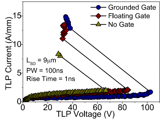
Figure 4. Comparison of TLP characteristics of AlGaIn/GaN HEMTs with and w/o gate.
