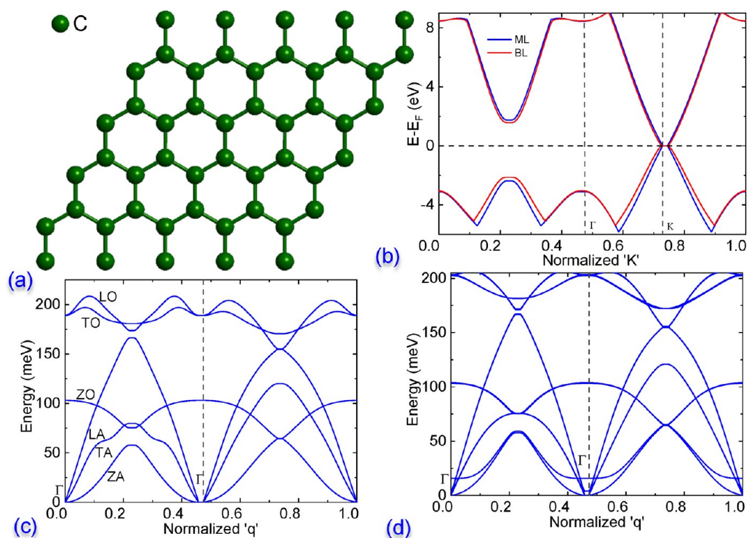
Figure 3. (a) Hexagonal lattice of graphene. (b) Electronic band structure of ML and BL graphene. Phonon band structure of (c) ML graphene and (d) BL graphene.
