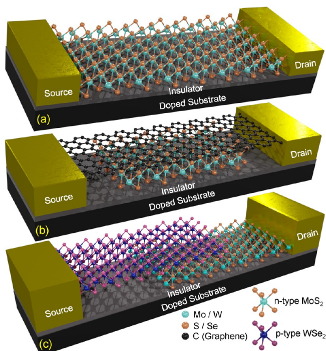
Figure 13. Isometric (atomistic) view of (a) 2D TMDC channel-based photodetector, (b) graphene-TMDC based photodetector, and (c) 2D TMDC heterostructure based photodetector.
