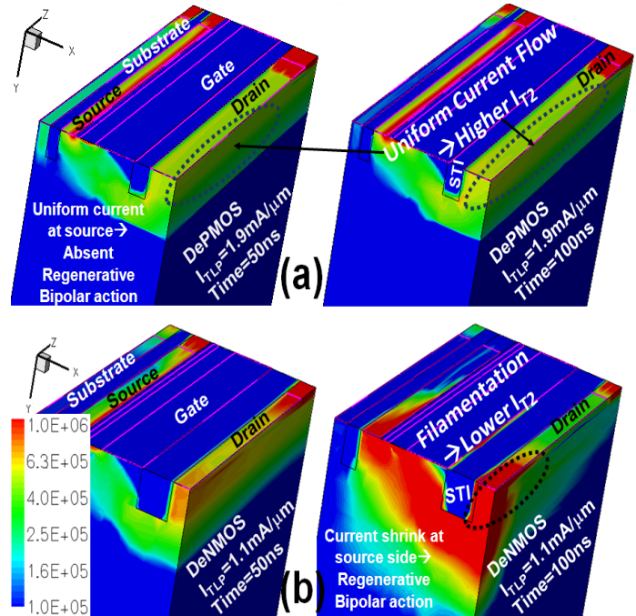
Fig. 7: Current Density Plot ( A/cm^2 ) for (a) DePMOS and (b) DeNMOS devices at different time.
