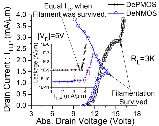
Fig. 10: Measured TLP characteristics of DeNMOS and DePMOS device at higher load line (i.e. R_L=3\text{k}\Omega ). Larger load survives the filamentation and leads to higher (almost equal) I_{T2} for both the devices.
