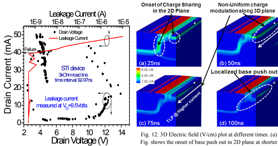
Fig. 11: TLP behavior of device at higher load line, i.e. 3kΩ. The figure shows soft snapback but no failure even up-to higher currents i.e. higher failure threshold. (leakage current measured at 9.5V).
