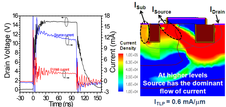
Fig. 5: At moderate/higher levels source current is dominant. This means that even though the device is in high resistance state at moderate/higher values of TLP pulse (Fig 2), the bipolar gets triggered efficiently
