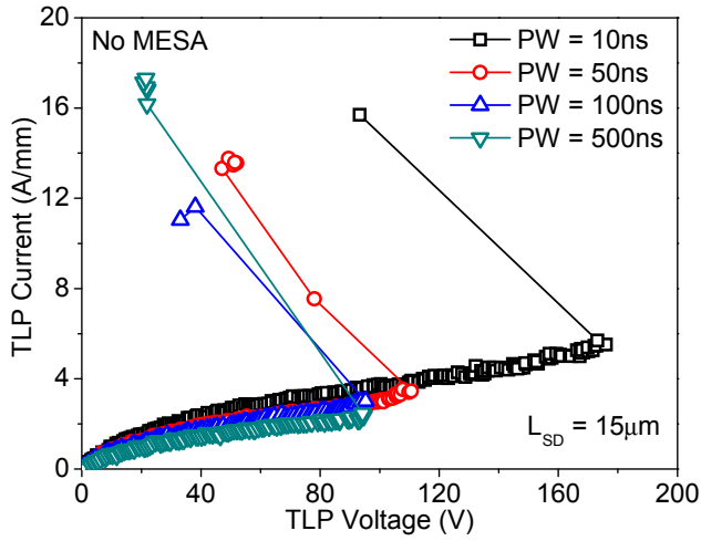
Figure 2: TLP characteristics of 50μm wide HEMTs without gate and MESA isolation with varying pulse width (PW). V_{SNAP} decreases and R_{ON} increases with increase in PW due to increased self heating in device.
