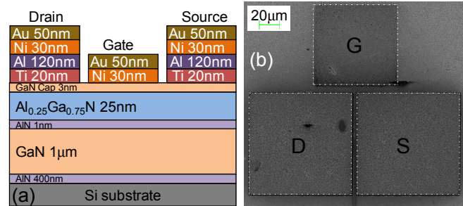
Figure 1: (a) Cross-sectional view of AlGaN/GaN HEMT with layer stack; and (b) SEM micrograph of the top view depicting gate finger between Source and Drain. Devices under stress are HEMTs w/ & w/o gate, w/ & w/o MESA and floating gate devices with different source-to-drain spacing ( L_{SD} ).
