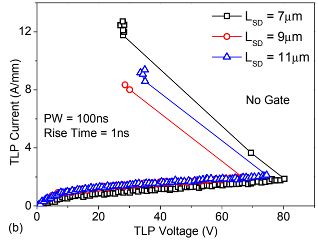
Figure 3: TLP characteristics of 100μm wide HEMTs without gate with varying (a) pulse width and (b) L_{SD} . Figure shows (a) decrease in V_{SNAP} and increase in R_{ON} with increase in PW due to increased device self heating & (b) improvement in V_{SNAP} with increase in L_{SD} at fixed PW = 100ns. Note: Device with L_{SD} = 7\mu m shows highest V_{SNAP} owing to its lowest On-current, attributed to device-to-device variability across wafer.
