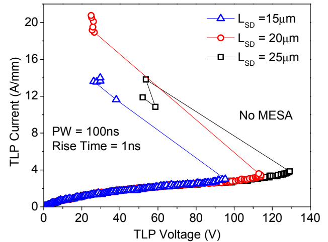
Figure 4: TLP characteristics of 50μm wide HEMTs without gate and MESA isolation with varying L_{SD} . V_{SNAP} increases with L_{SD} .
