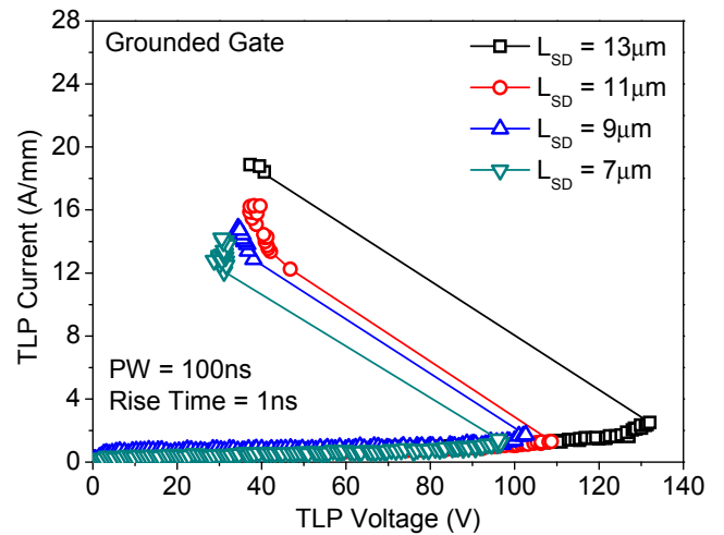
Figure 7: TLP characteristics of 100 \mu m wide HEMTs with different L_{SD} under grounded gate configuration. Note that V_{SNAP} and failure current ( I_{T2} ) increase with L_{SD} .
