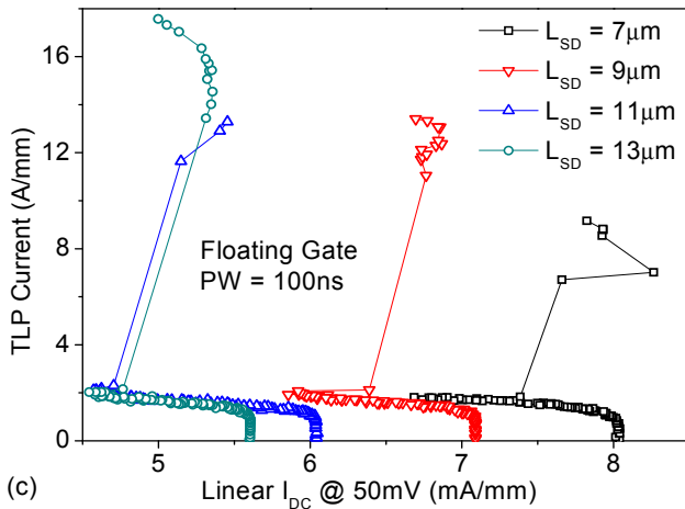
Figure 5: TLP characteristics of 100 \mu m wide HEMTs with gate floating with varying (a) pulse width and (b) L_{SD} . Figure shows (i) decrease in V_{SNAP} and increase in R_{ON} with increase in pulse width due to higher self heating; (ii) increase in V_{SNAP} and I_{FAIL} with L_{SD} (c) leakage (here linear drain current) / spot measurements depicting (i) device failure point and (ii) device degradation after every stress pulse.
