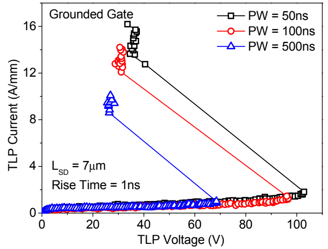
Figure 6: TLP characteristics of 100 \mu m wide HEMTs with varying PW under grounded gate configuration.
