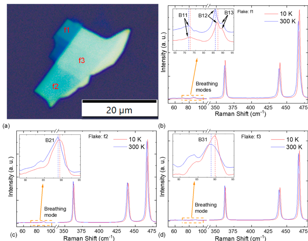
Figure 4. (a) Phosphorene flake has different thickness regions (f1, f2, and f3), captured using an OLYMPUS BX53M microscope with 100× objective. (b–d) Raman spectra of the regions f1, f2, and f3, respectively, at 10 and 300 K. Breathing modes of all the flakes are named in the insets.
